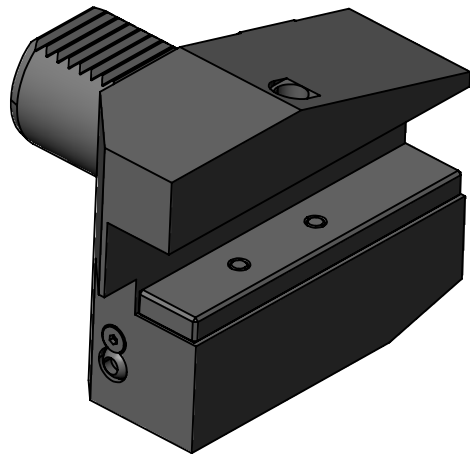
90 DEGREE VDI40 STATIC TOOL OUTPUT: 1" SQR SHANK COOLANT: EXTERNAL
